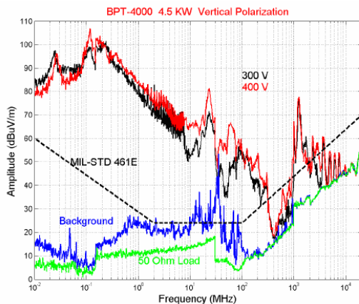
Fig. 1. Example of vertically polarized emission spectra from BPT-4000 operating at 4.5 kW [2].
