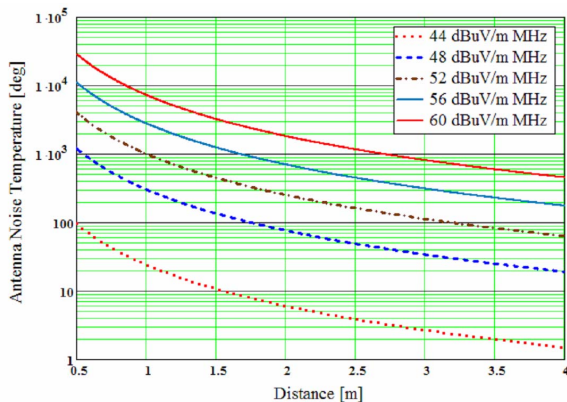
Fig. 3. Noise temperature as a function of EP distance
