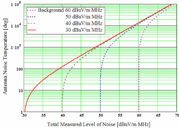
Fig. 2. Noise temperature as a function of measured noise signal at the antenna input
