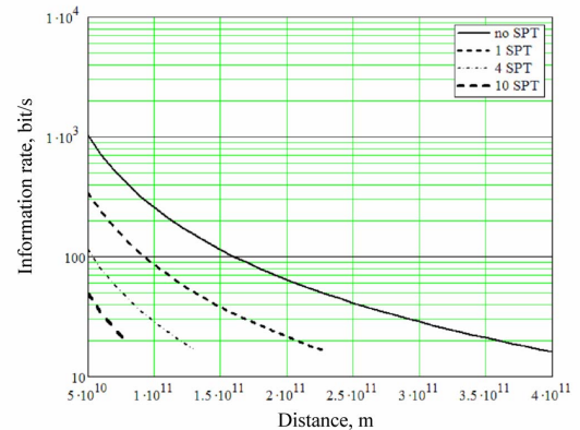
Fig. 5. Information rate as a function of communication range
